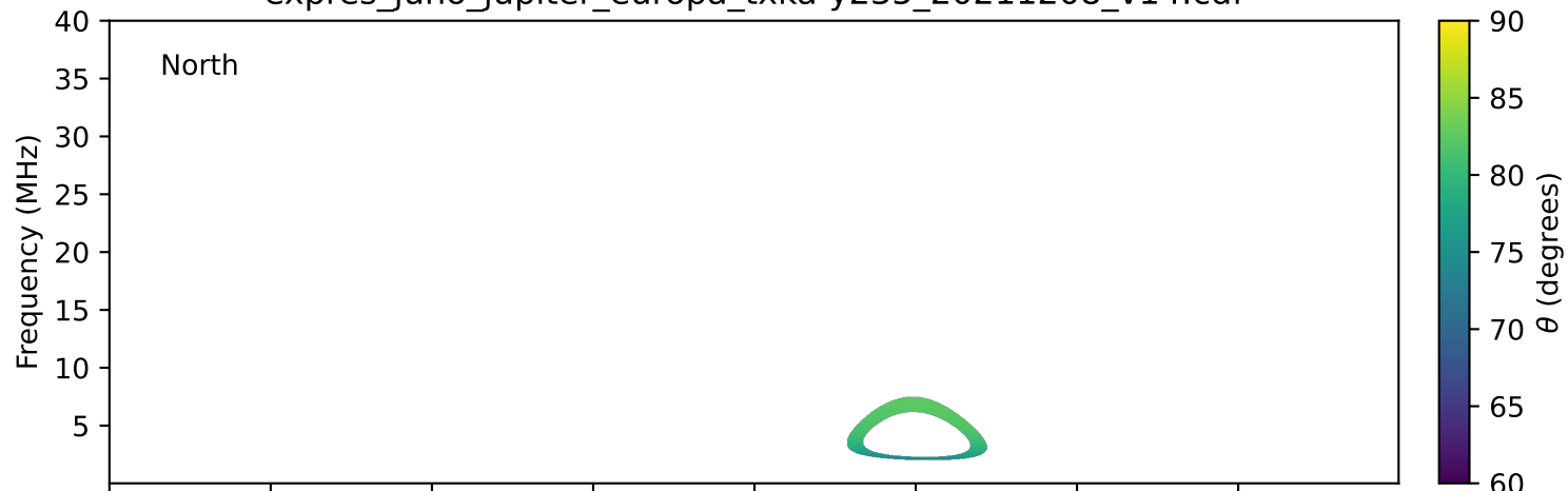
expres_juno_jupiter_europa_txka-y235_20211208_v14.cdf
