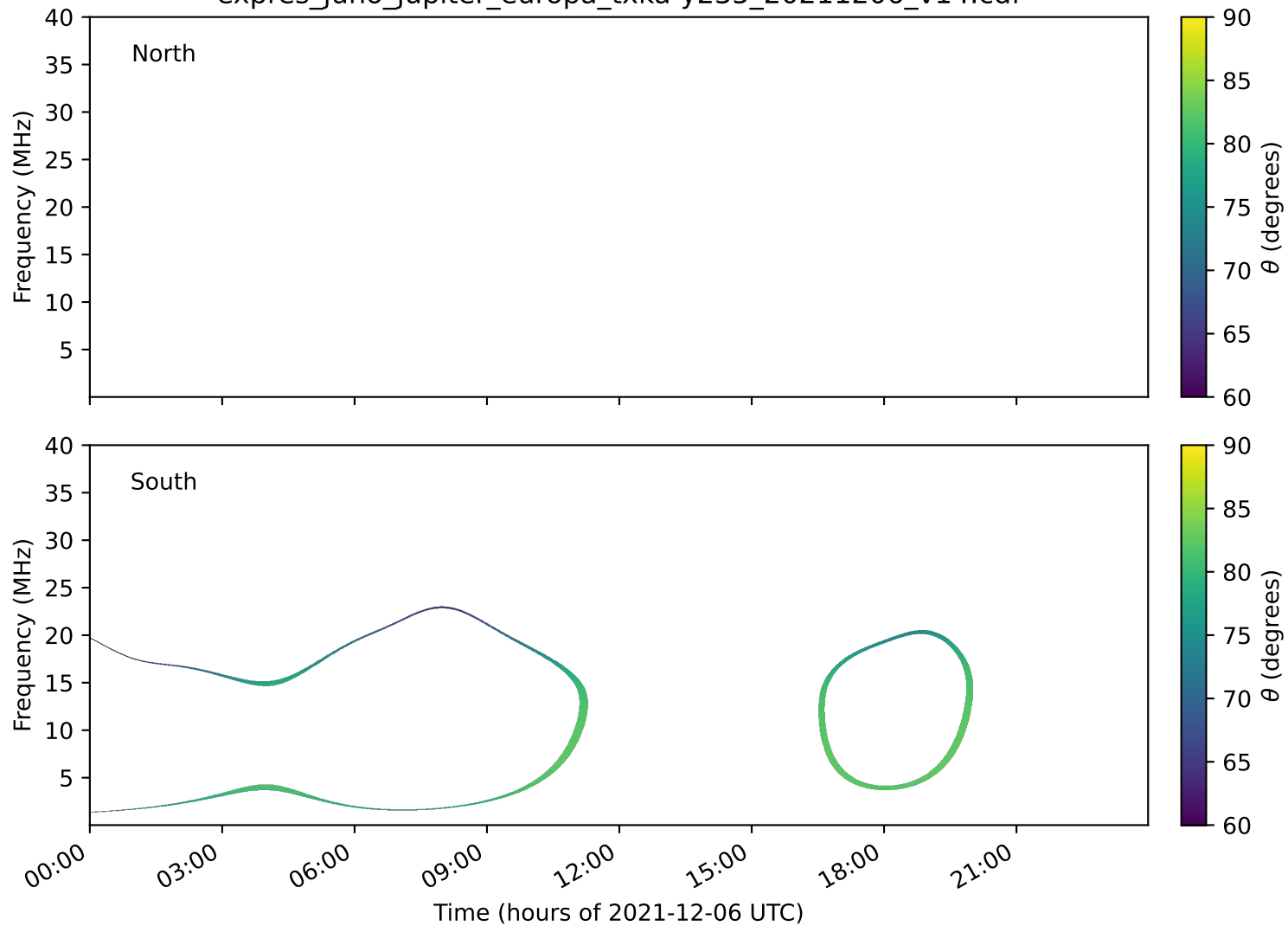
expres_juno_jupiter_europa_txka-y235_20211206_v14.cdf
