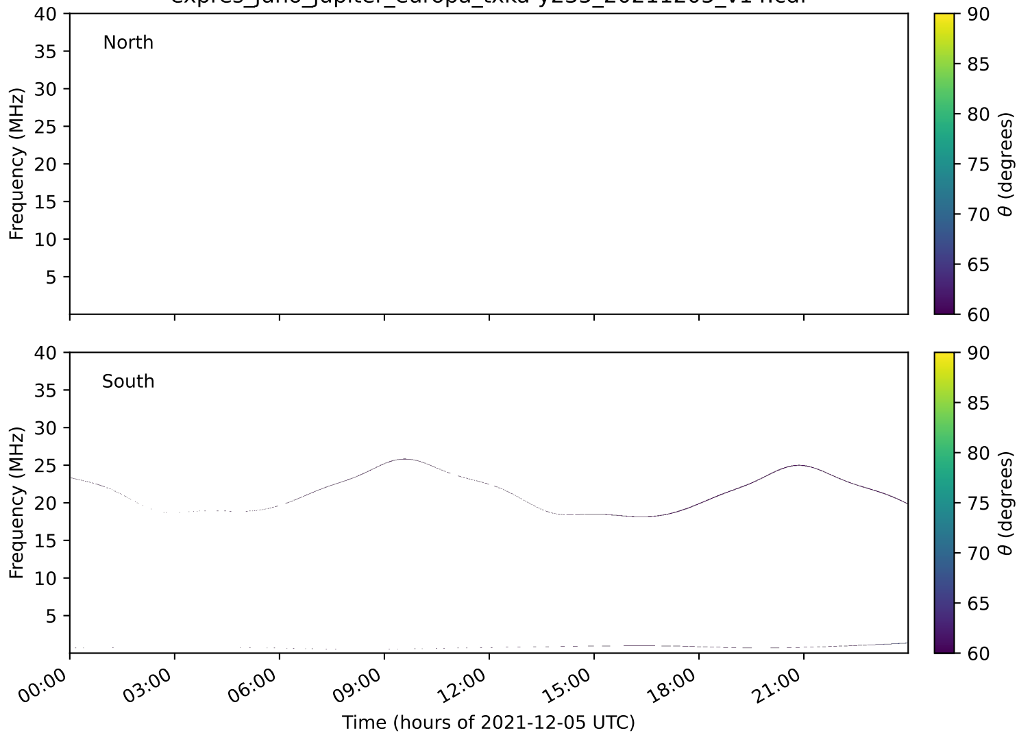
expres_juno_jupiter_europa_txka-y235_20211205_v14.cdf
