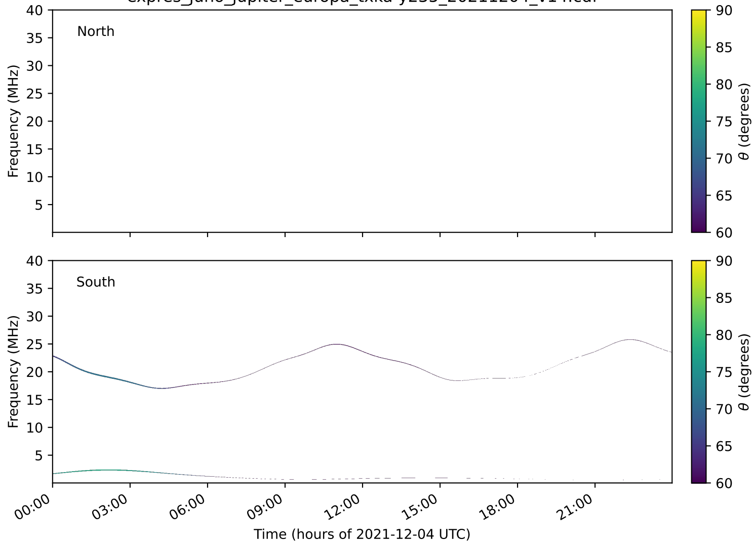
expres_juno_jupiter_europa_txka-y235_20211204_v14.cdf
