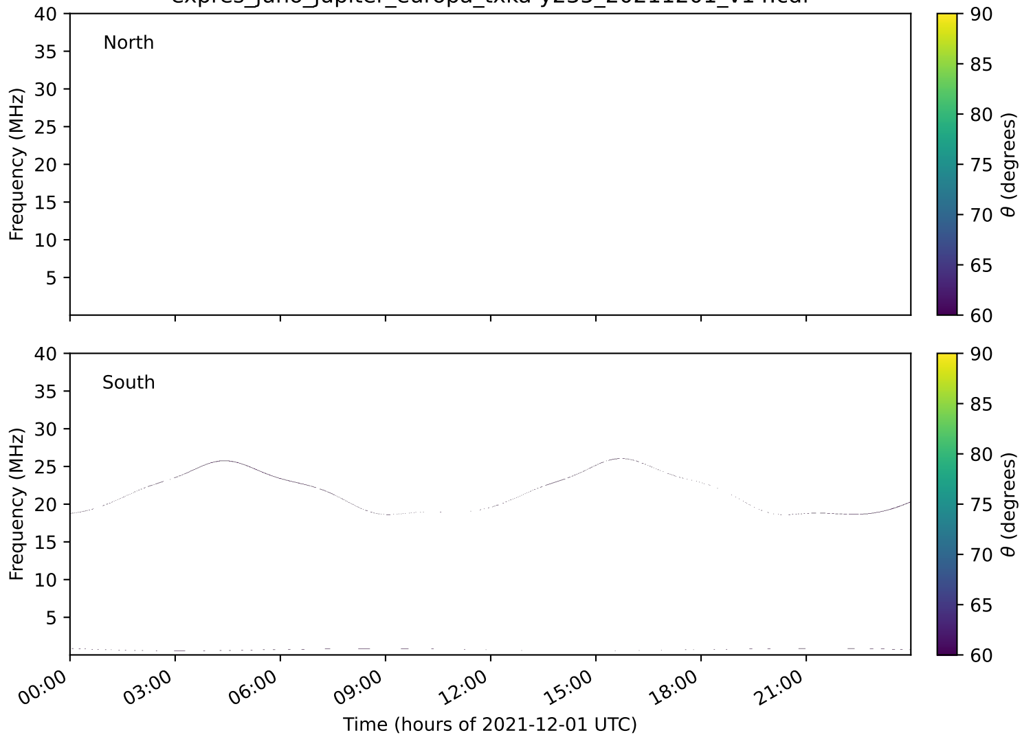
expres_juno_jupiter_europa_txka-y235_20211201_v14.cdf
