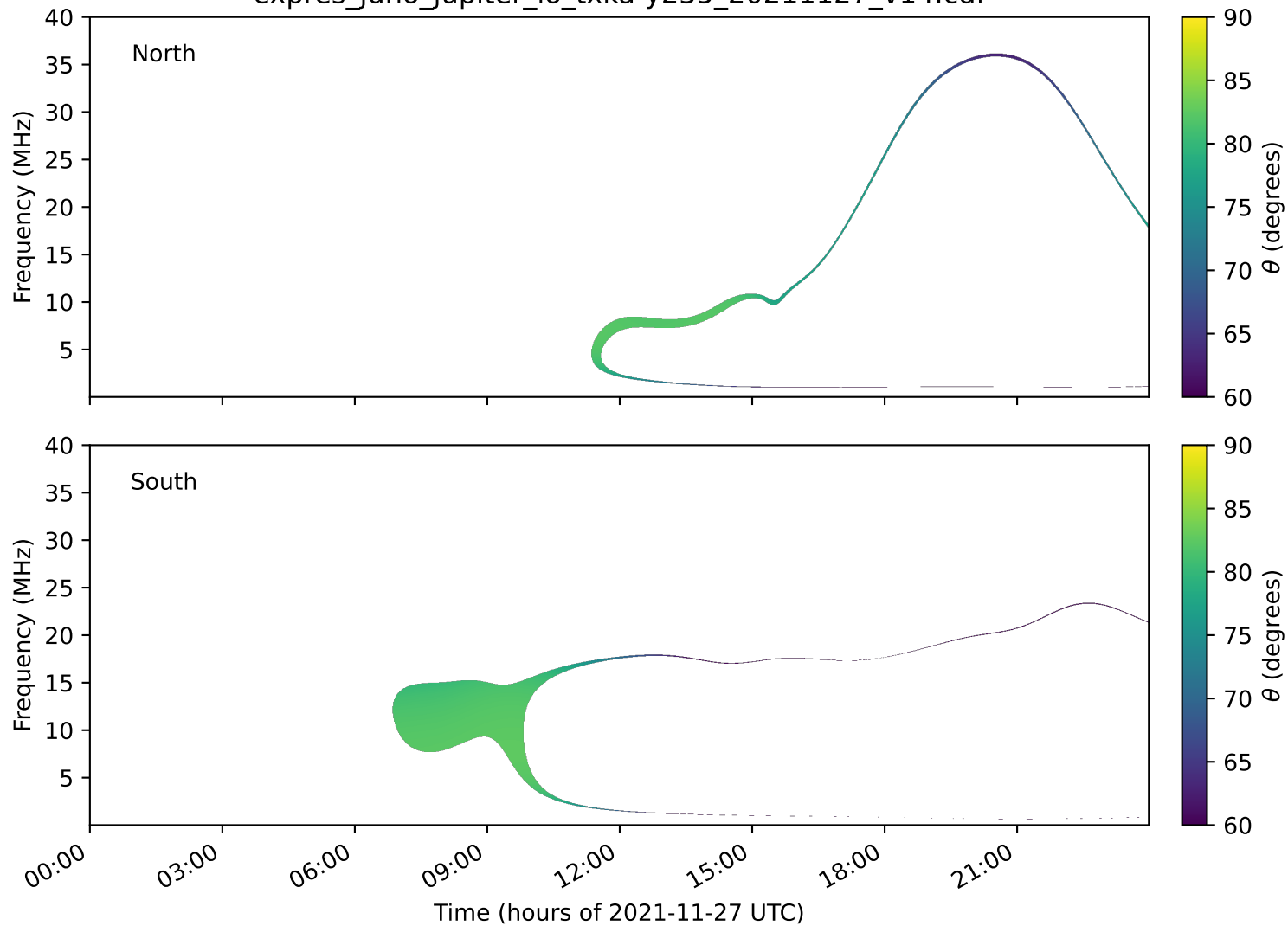
expres_juno_jupiter_io_txka-y235_20211127_v14.cdf
