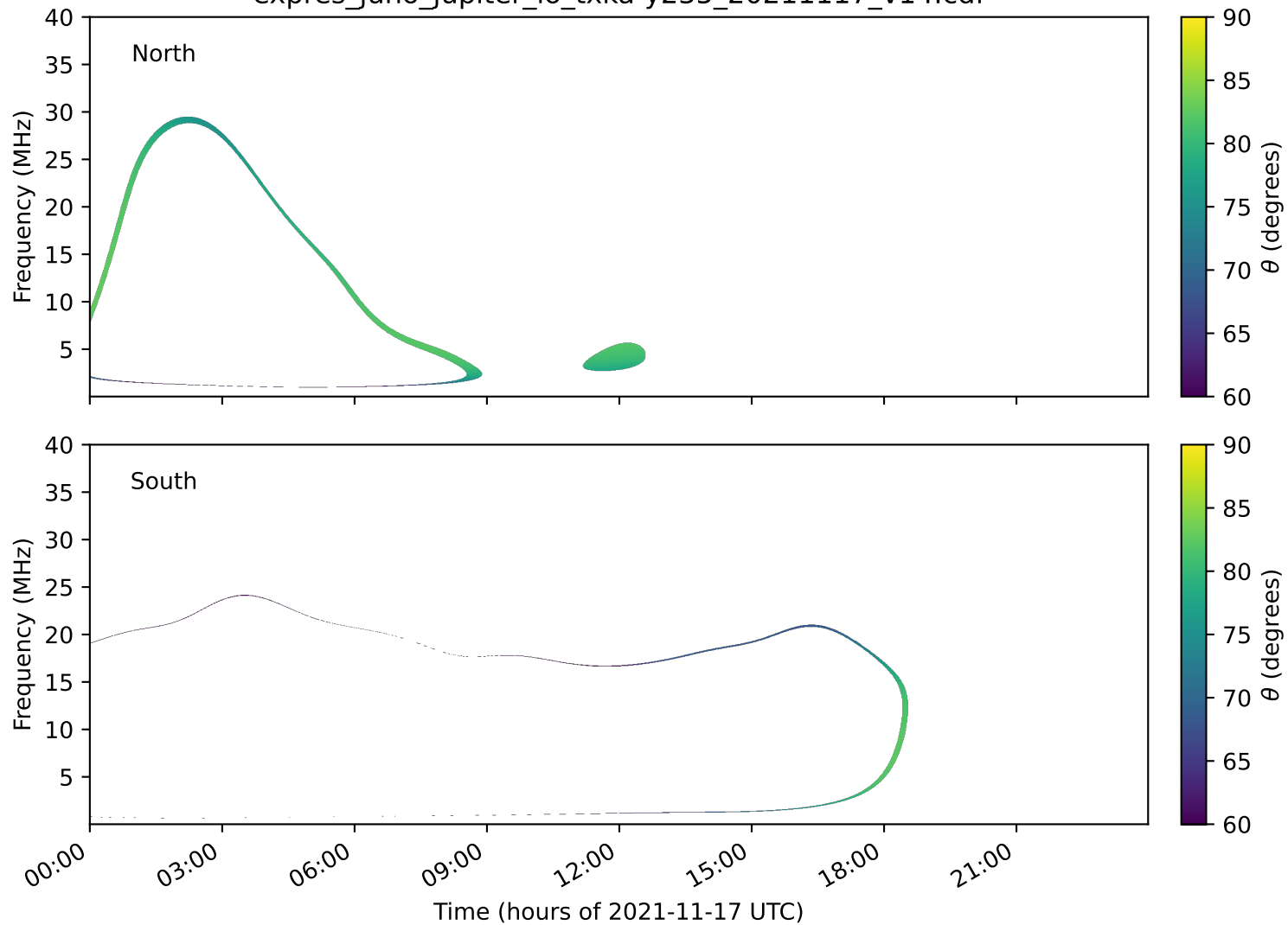
expres_juno_jupiter_io_txka-y235_20211117_v14.cdf
