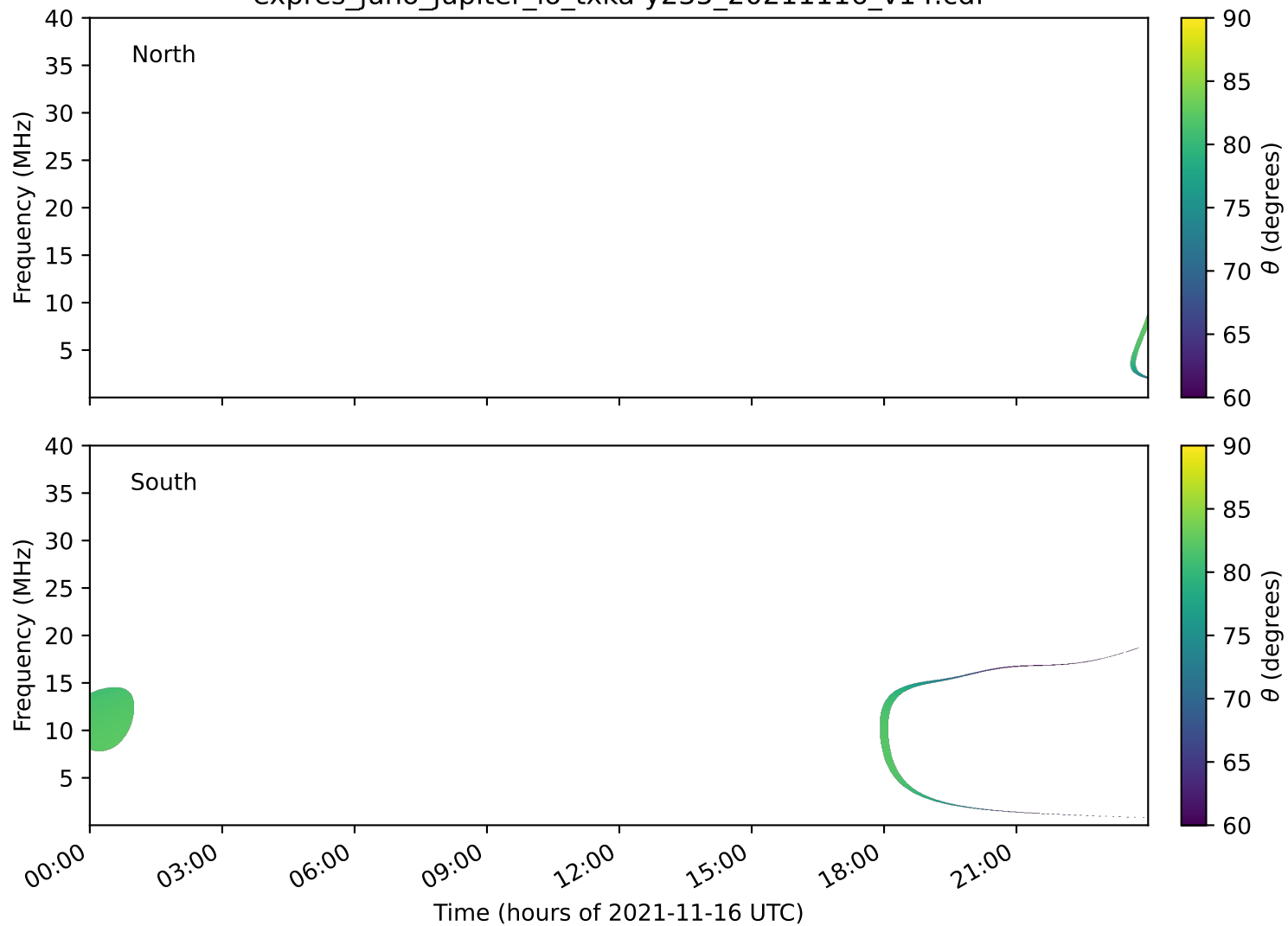
expres_juno_jupiter_io_txka-y235_20211116_v14.cdf
