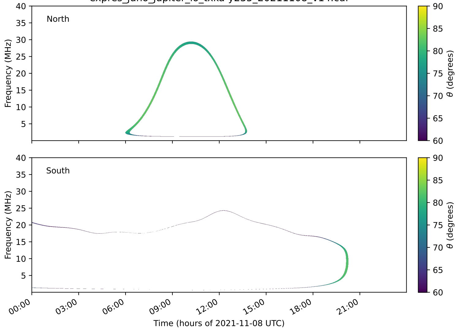
expres_juno_jupiter_io_txka-y235_20211108_v14.cdf
