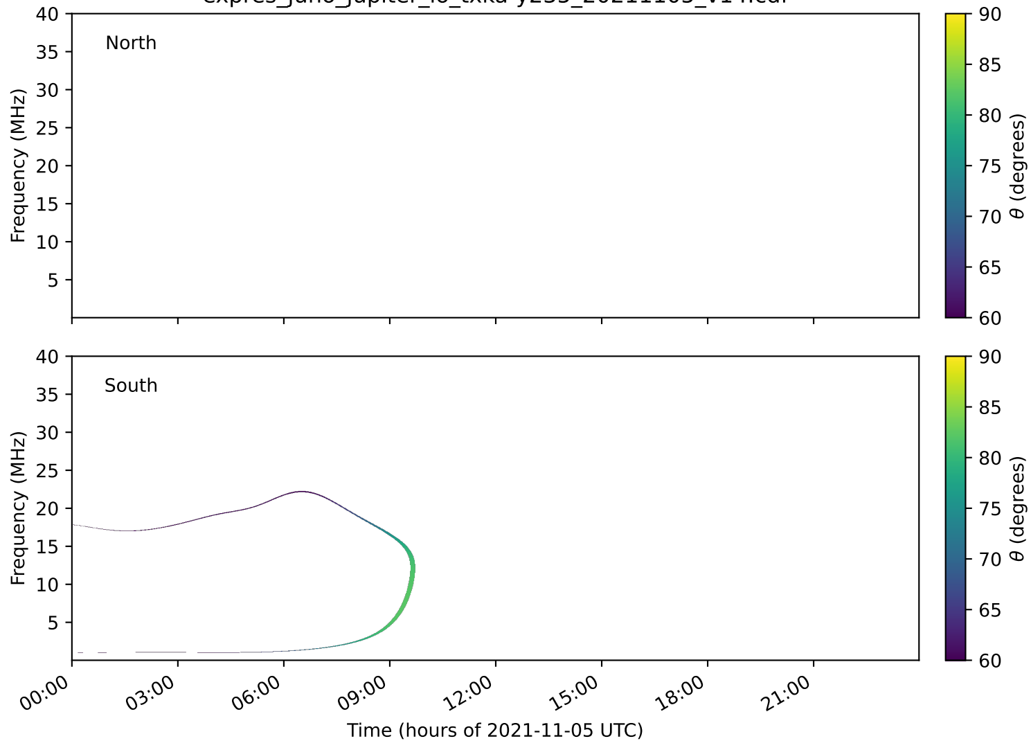
expres_juno_jupiter_io_txka-y235_20211105_v14.cdf
