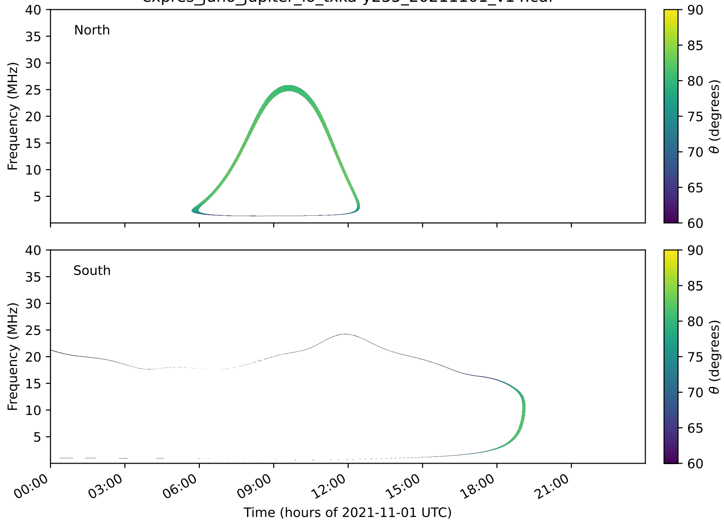
expres_juno_jupiter_io_txka-y235_20211101_v14.cdf
