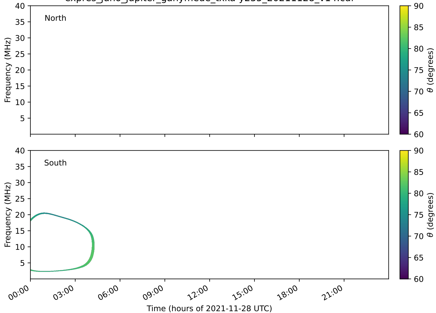
expres_juno_jupiter_ganymede_txka-y235_20211128_v14.cdf
