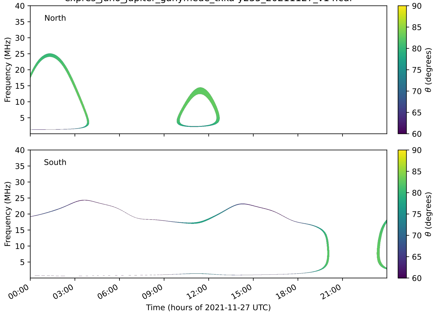
expres_juno_jupiter_ganymede_txka-y235_20211127_v14.cdf
