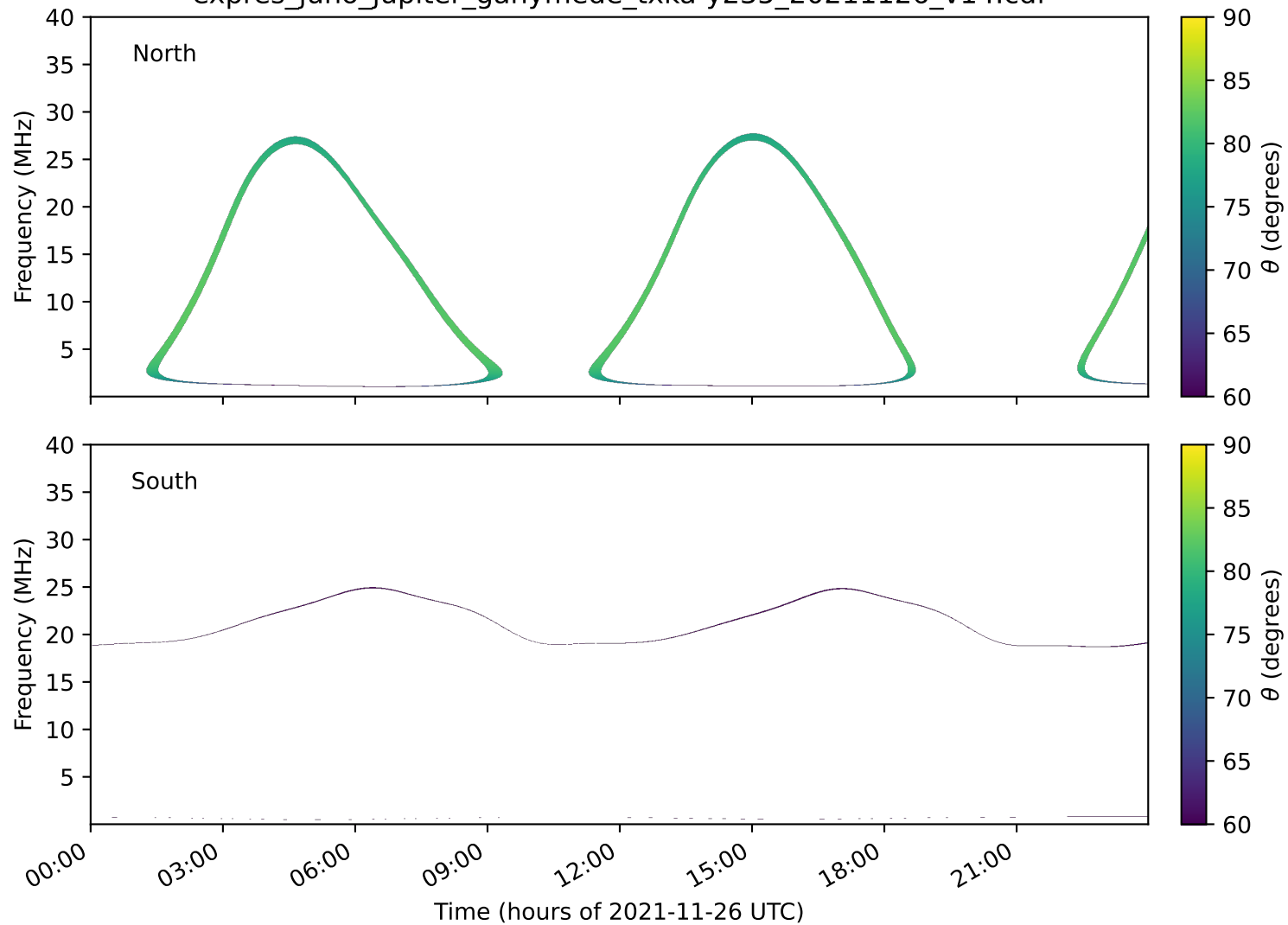
expres_juno_jupiter_ganymede_txka-y235_20211126_v14.cdf
