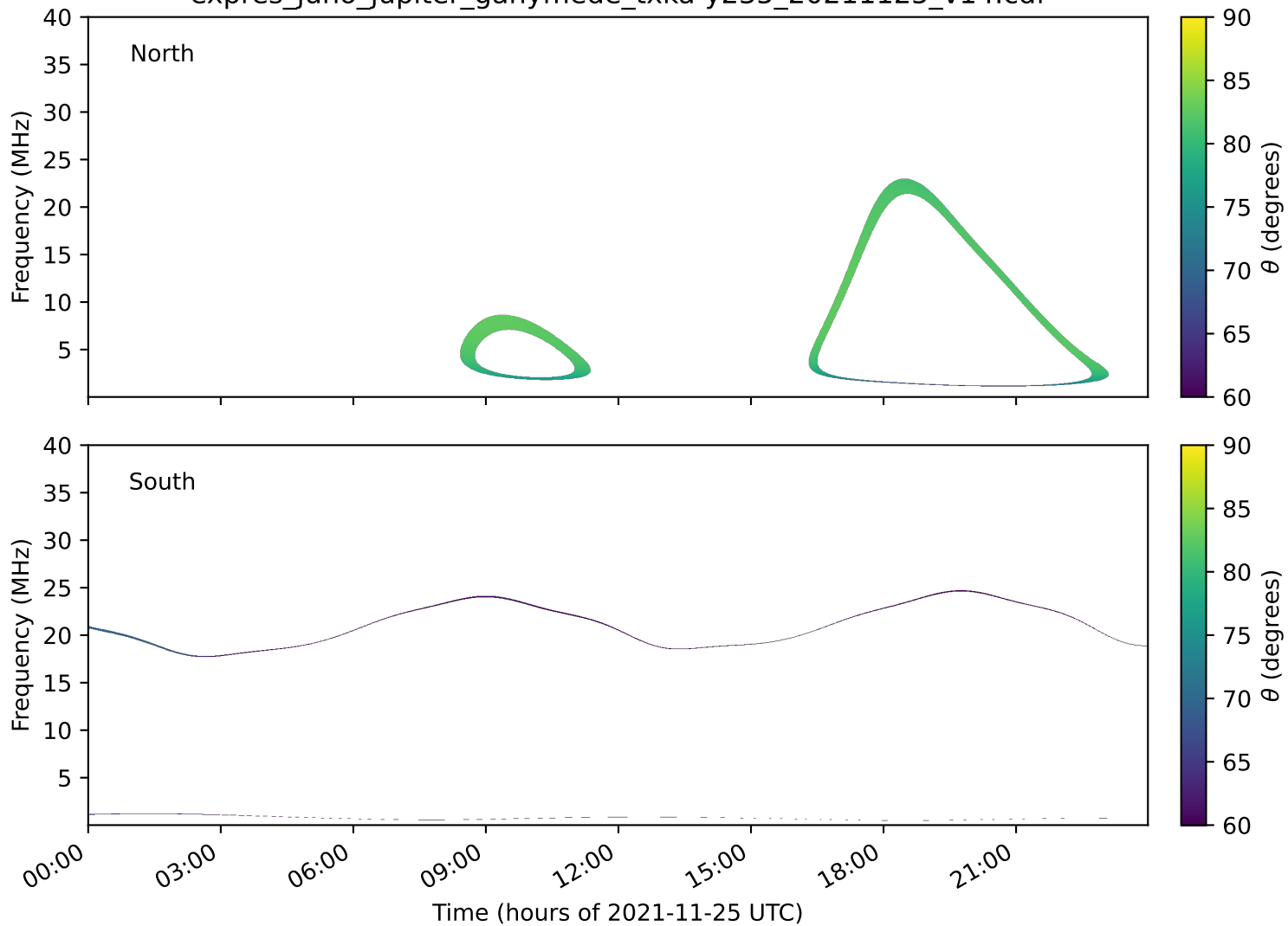
expres_juno_jupiter_ganymede_txka-y235_20211125_v14.cdf
