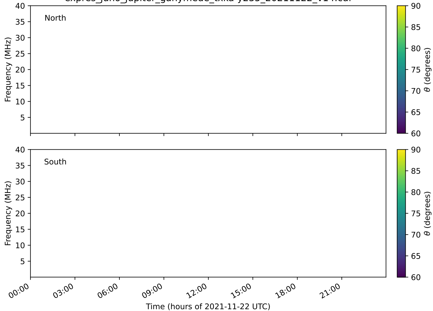
expres_juno_jupiter_ganymede_txka-y235_20211122_v14.cdf
