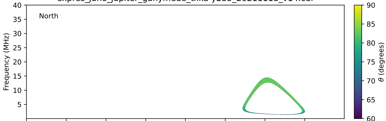
expres_juno_jupiter_ganymede_txka-y235_20211118_v14.cdf
