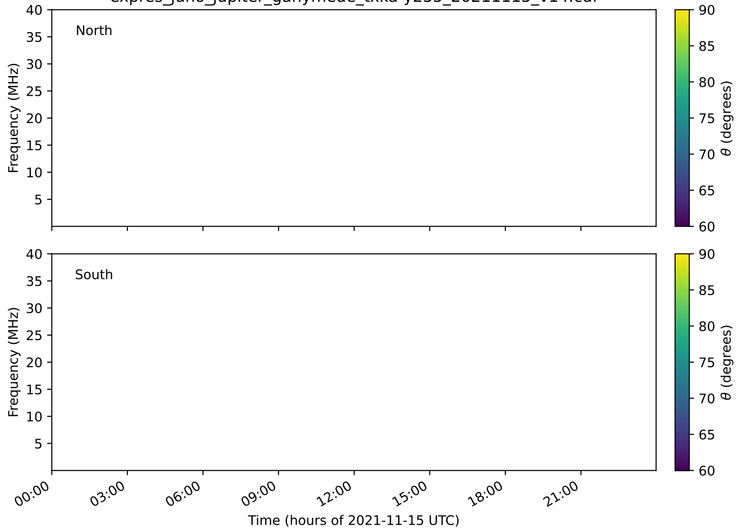
expres_juno_jupiter_ganymede_txka-y235_20211115_v14.cdf
