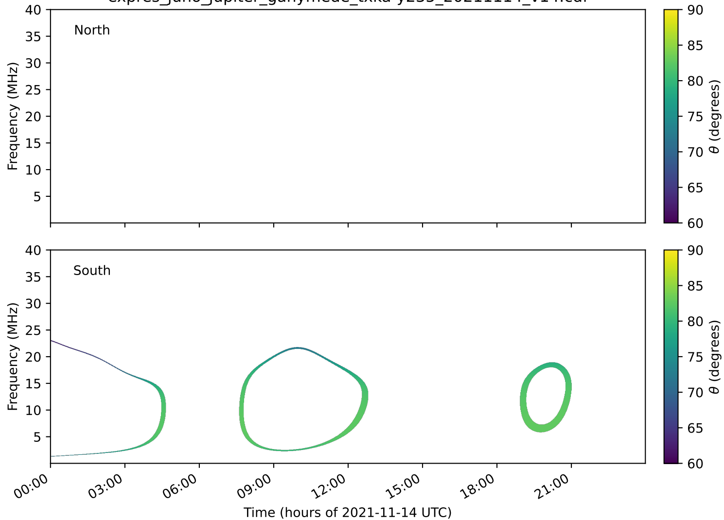
expres_juno_jupiter_ganymede_txka-y235_20211114_v14.cdf
