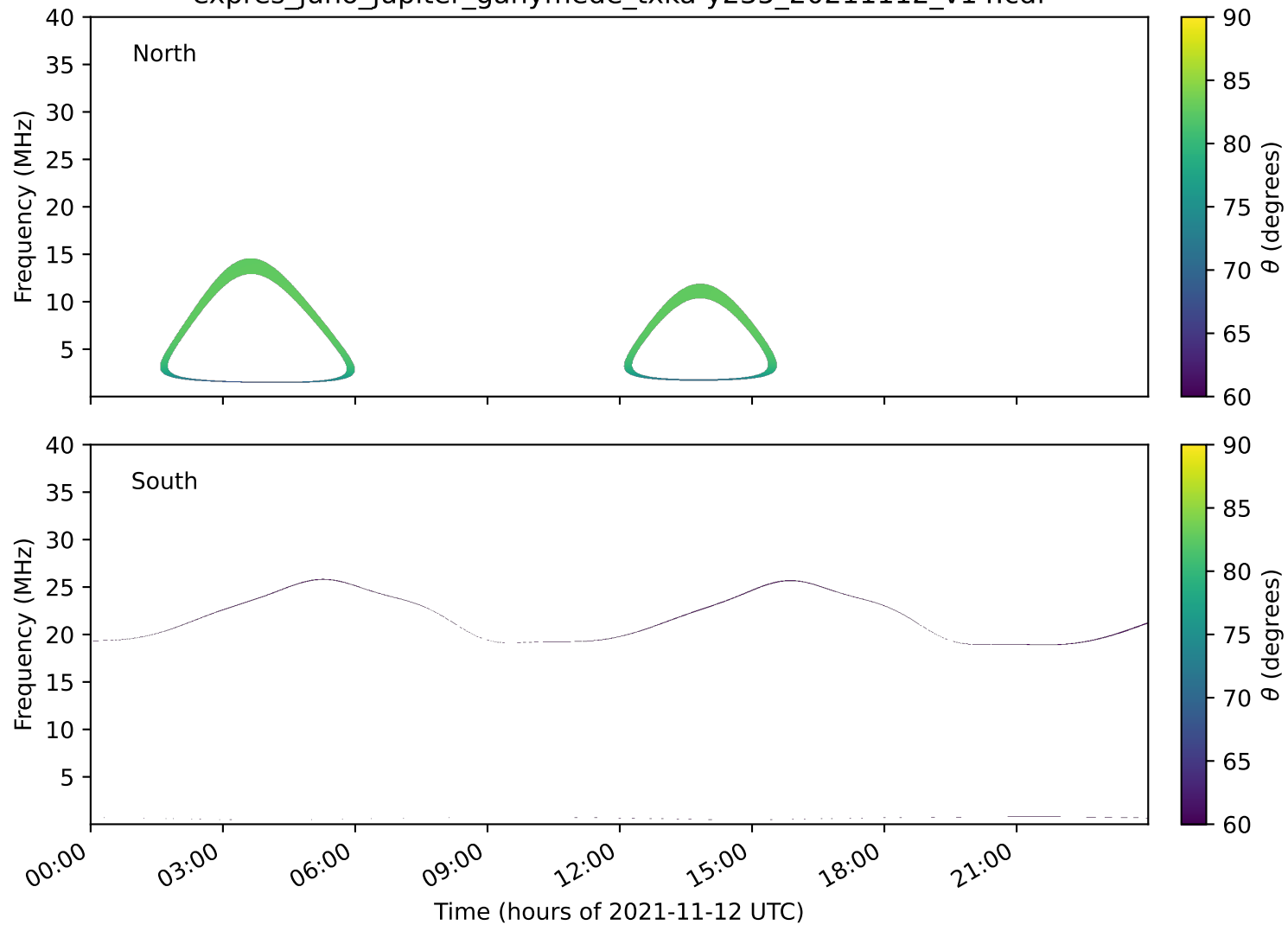
expres_juno_jupiter_ganymede_txka-y235_20211112_v14.cdf
