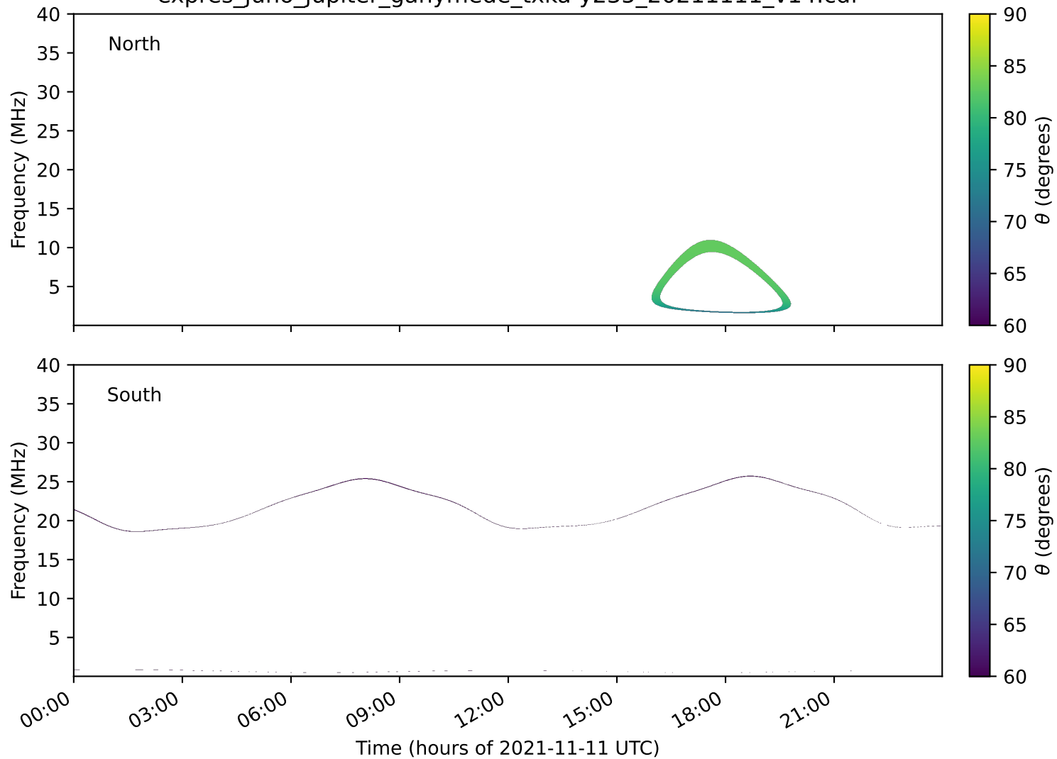
expres_juno_jupiter_ganymede_txka-y235_20211111_v14.cdf
