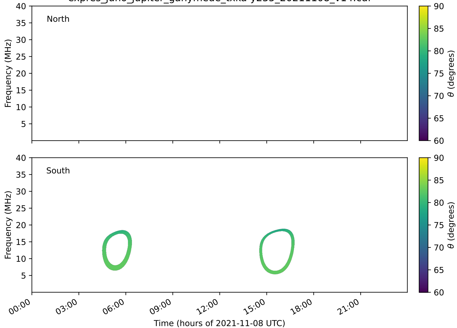
expres_juno_jupiter_ganymede_txka-y235_20211108_v14.cdf
