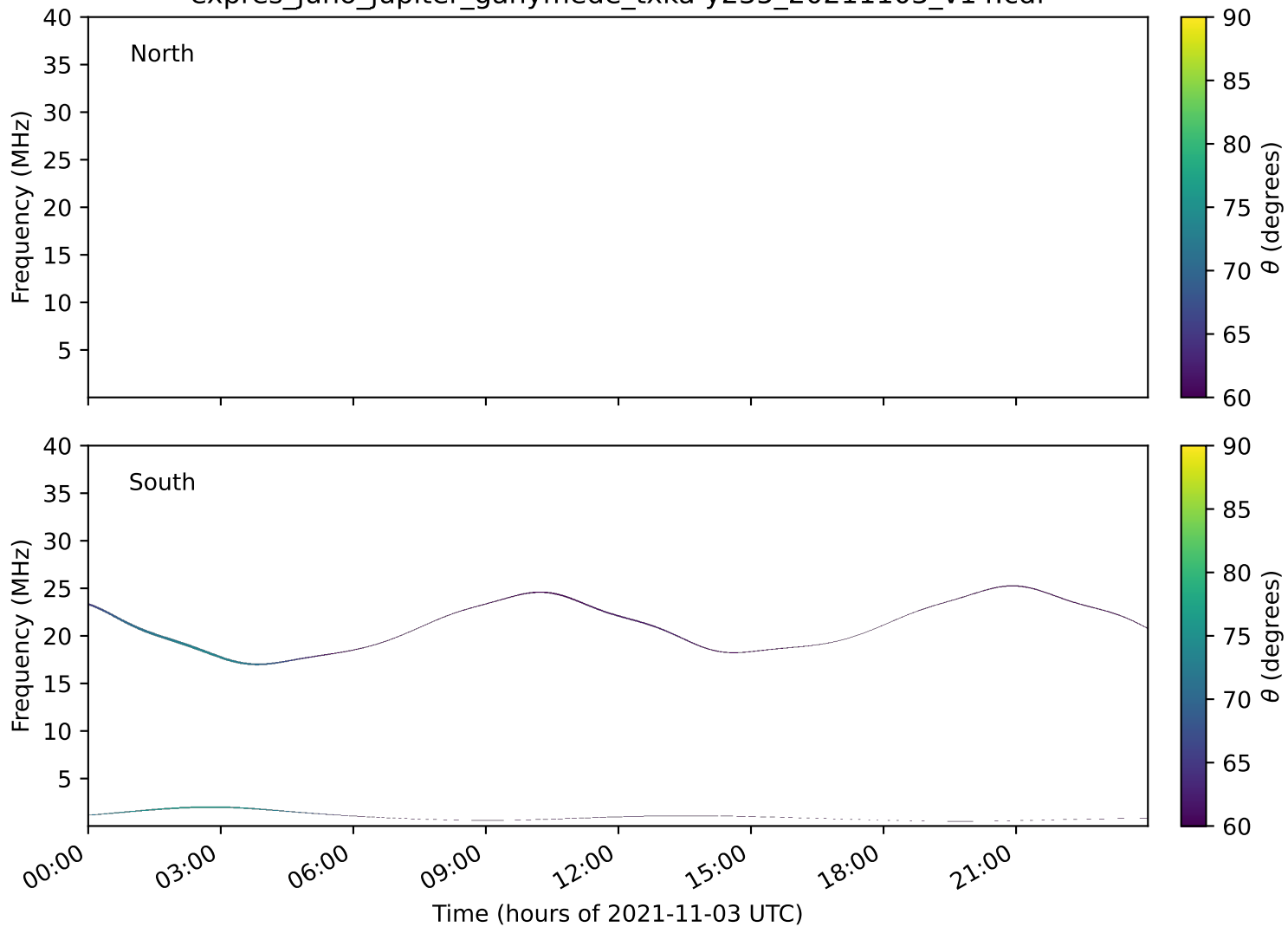
expres_juno_jupiter_ganymede_txka-y235_20211103_v14.cdf
