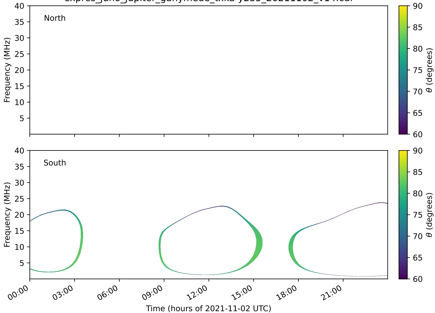
expres_juno_jupiter_ganymede_txka-y235_20211102_v14.cdf
