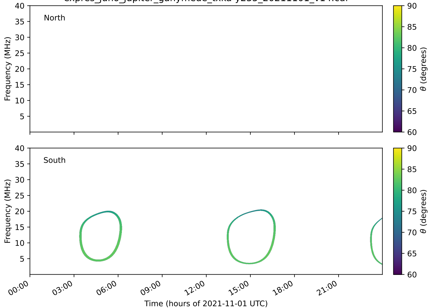
expres_juno_jupiter_ganymede_txka-y235_20211101_v14.cdf
