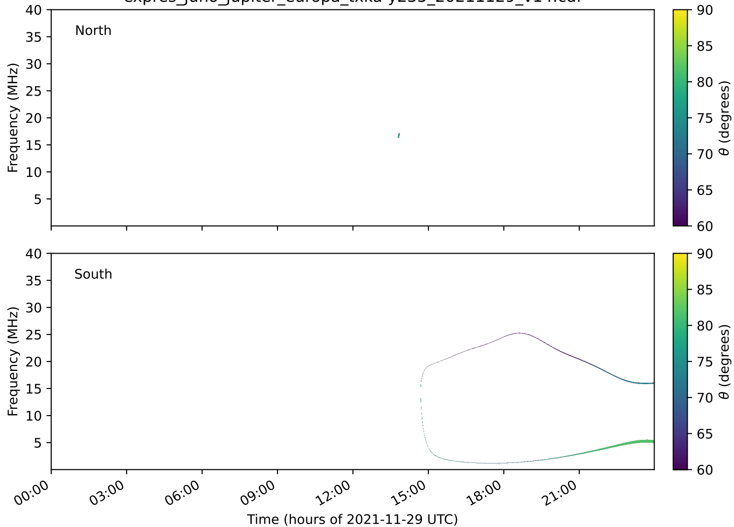
expres_juno_jupiter_europa_txka-y235_20211129_v14.cdf
