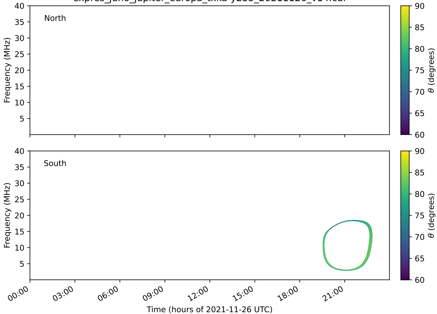
expres_juno_jupiter_europa_txka-y235_20211126_v14.cdf
