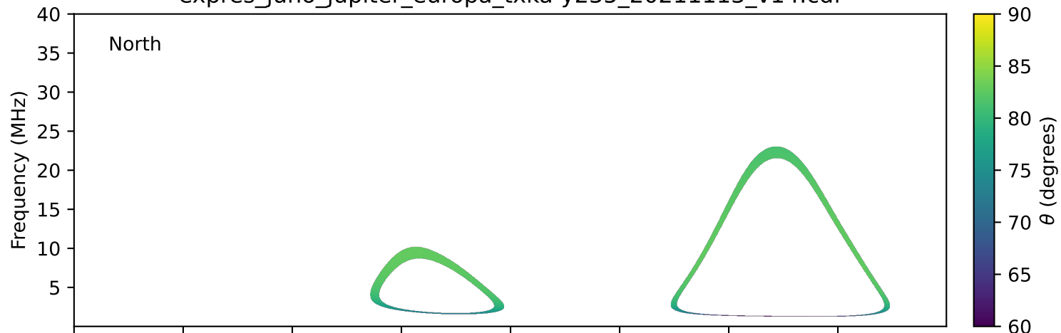
expres_juno_jupiter_europa_txka-y235_20211113_v14.cdf
