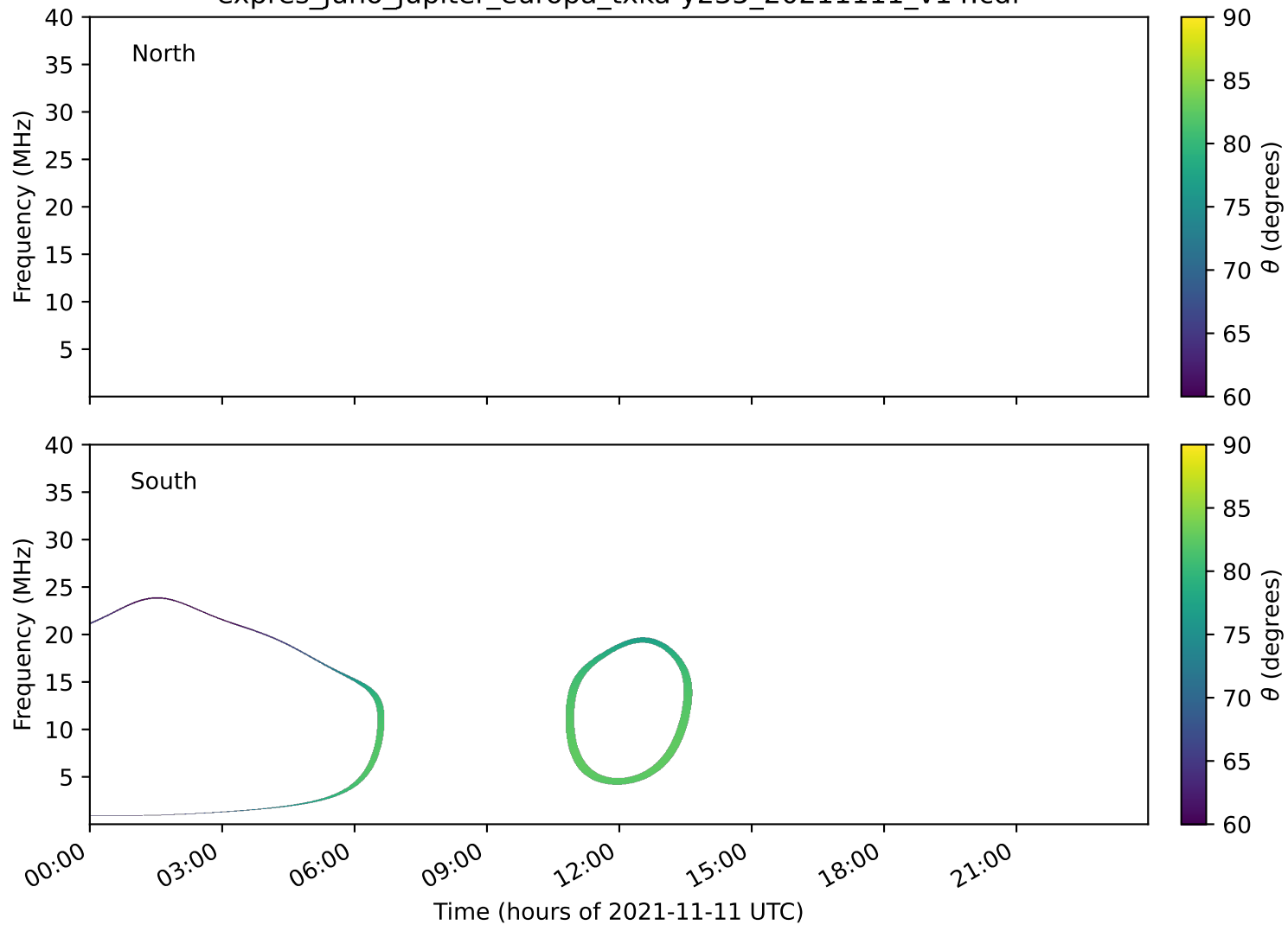
expres_juno_jupiter_europa_txka-y235_20211111_v14.cdf
