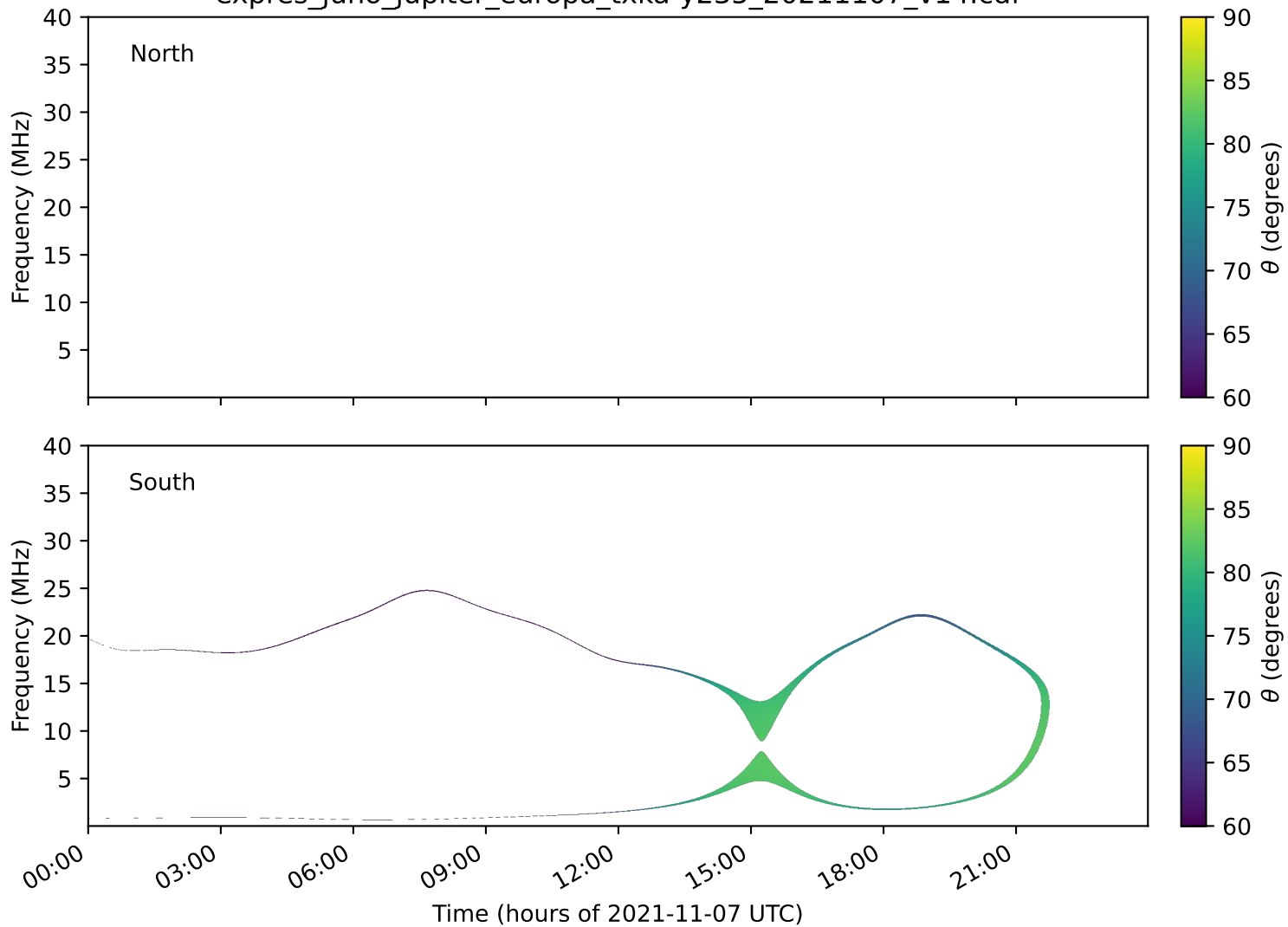
expres_juno_jupiter_europa_txka-y235_20211107_v14.cdf
