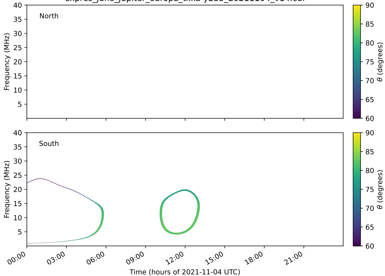
expres_juno_jupiter_europa_txka-y235_20211104_v14.cdf
