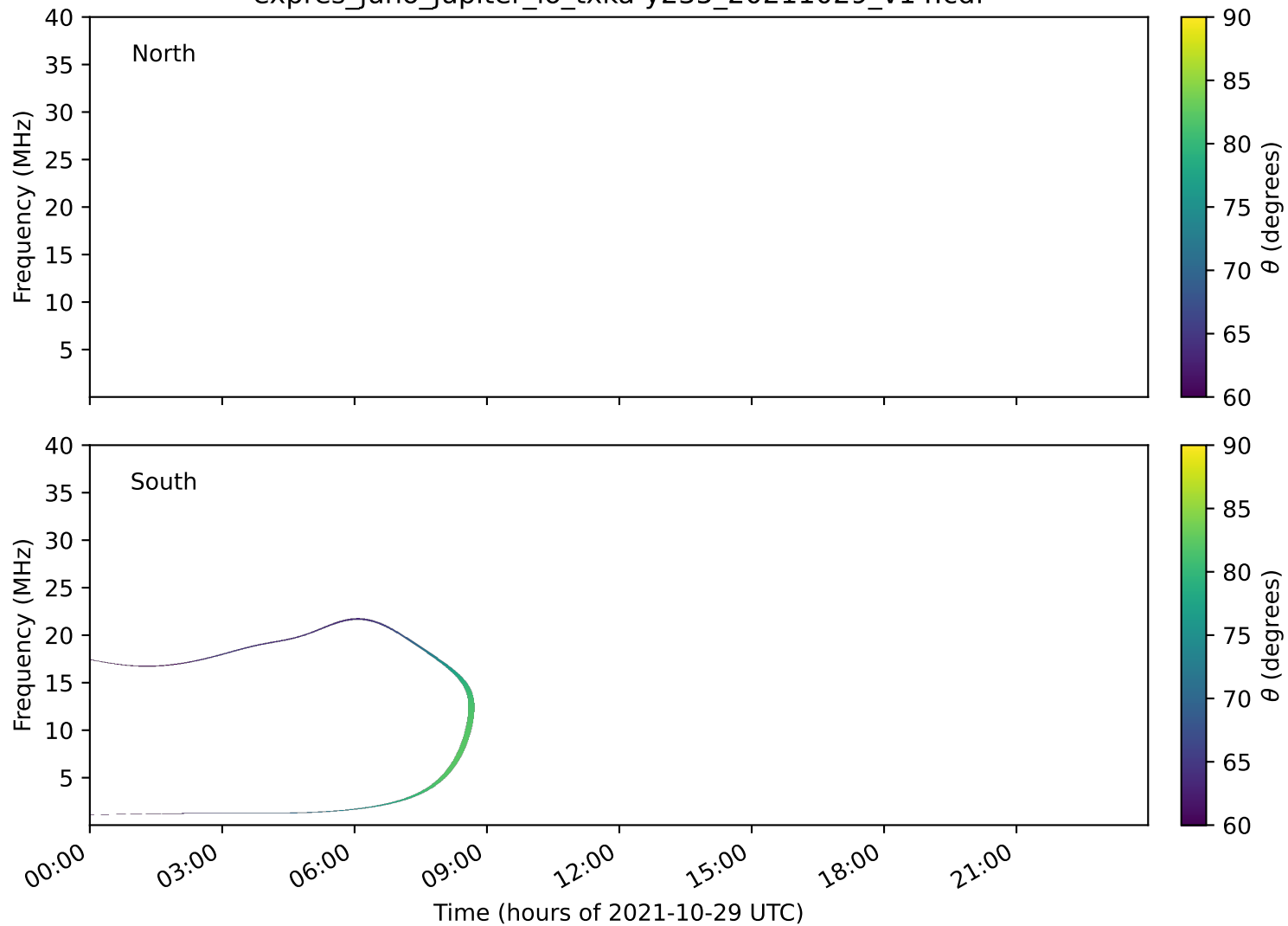
expres_juno_jupiter_io_txka-y235_20211029_v14.cdf
