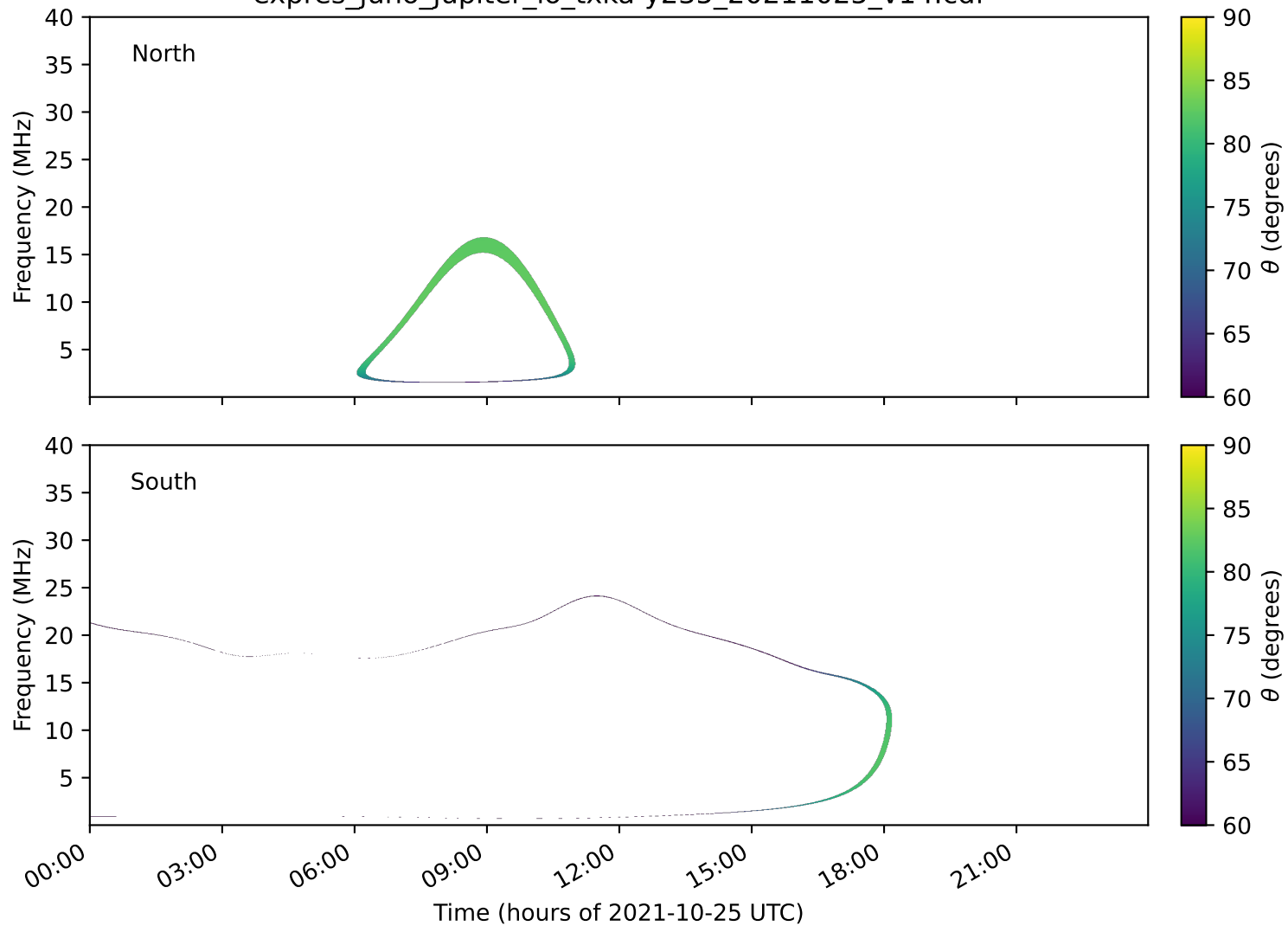
expres_juno_jupiter_io_txka-y235_20211025_v14.cdf
