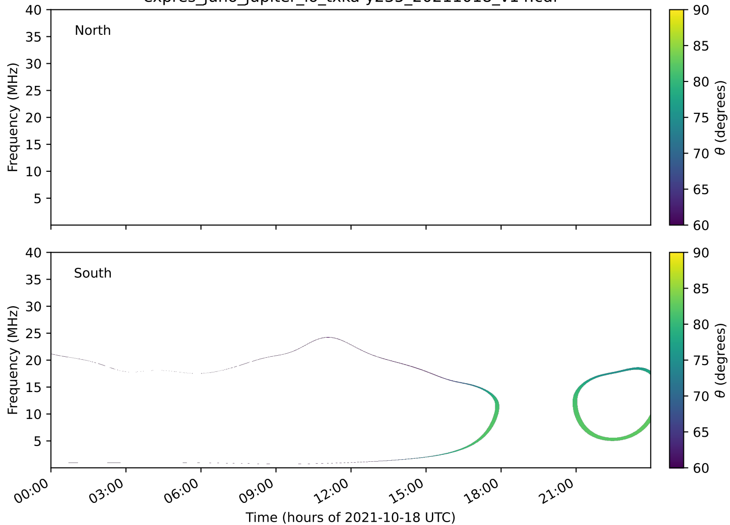
expres_juno_jupiter_io_txka-y235_20211018_v14.cdf
