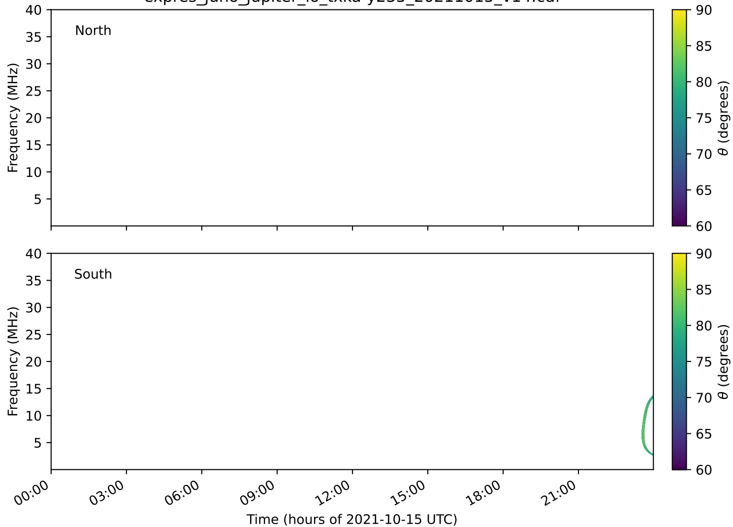
expres_juno_jupiter_io_txka-y235_20211015_v14.cdf
