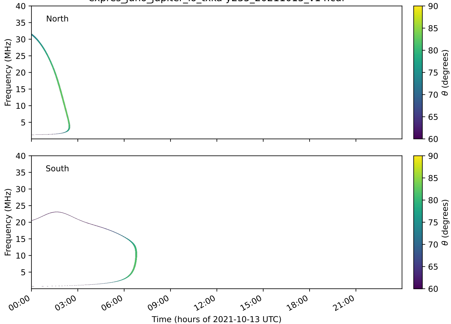
expres_juno_jupiter_io_txka-y235_20211013_v14.cdf
