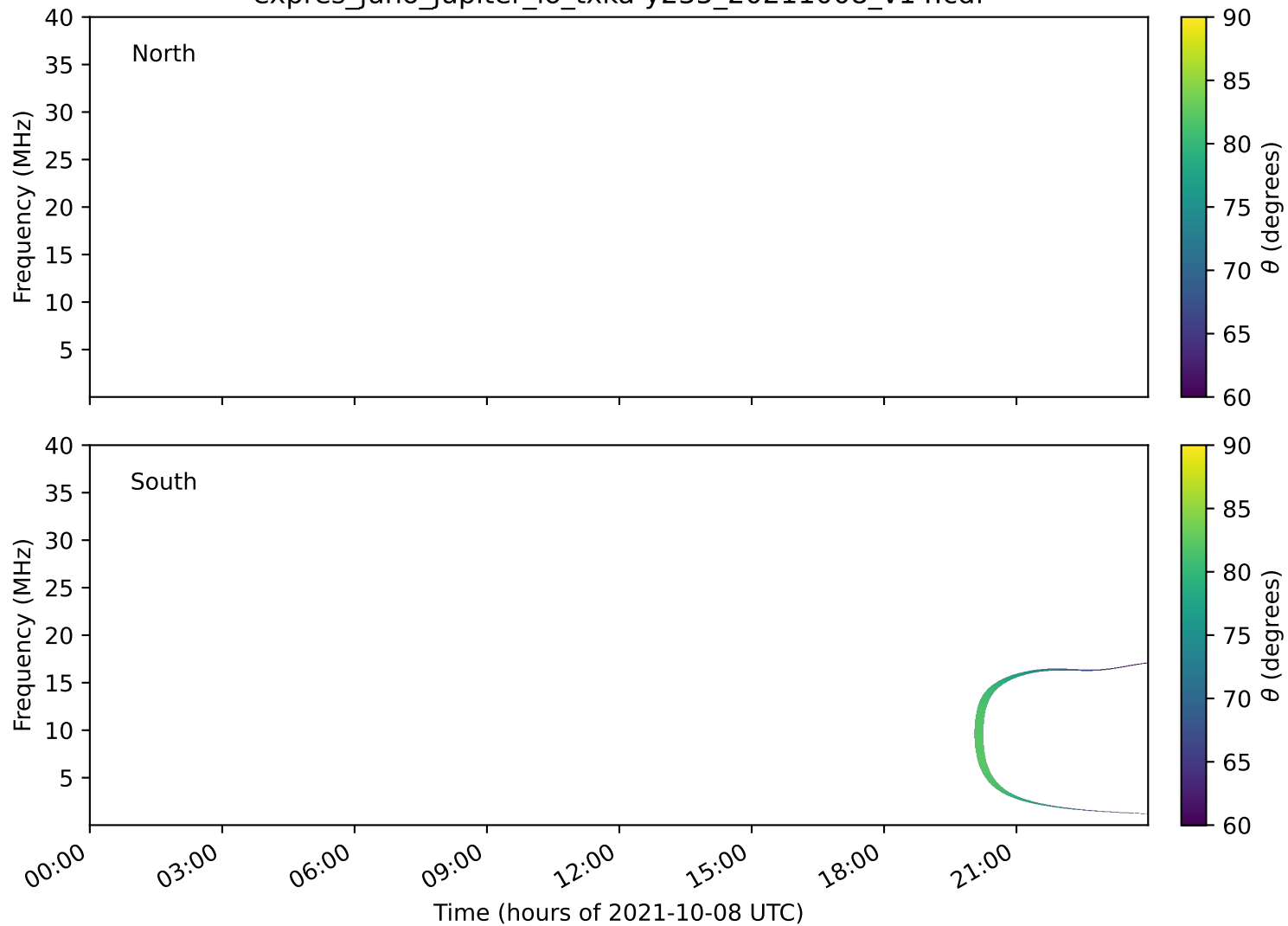
expres_juno_jupiter_io_txka-y235_20211008_v14.cdf
