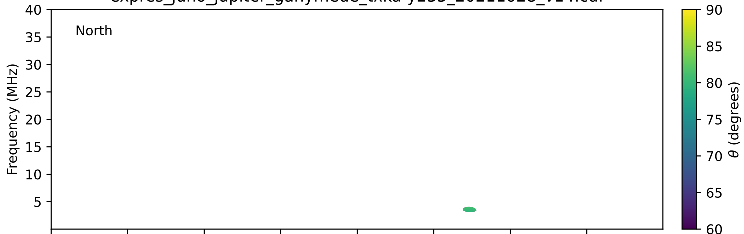
expres_juno_jupiter_ganymede_txka-y235_20211028_v14.cdf
