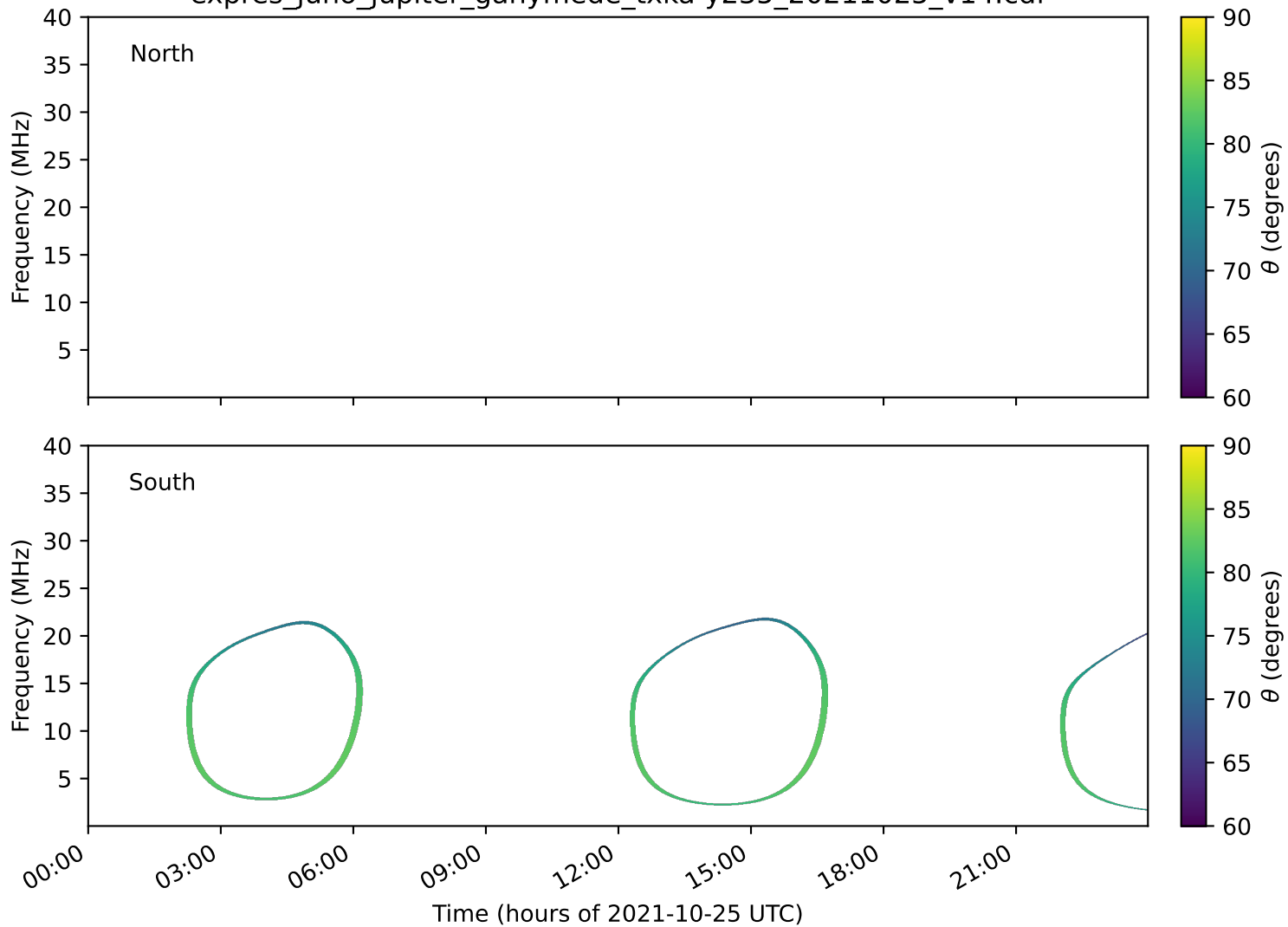
expres_juno_jupiter_ganymede_txka-y235_20211025_v14.cdf
