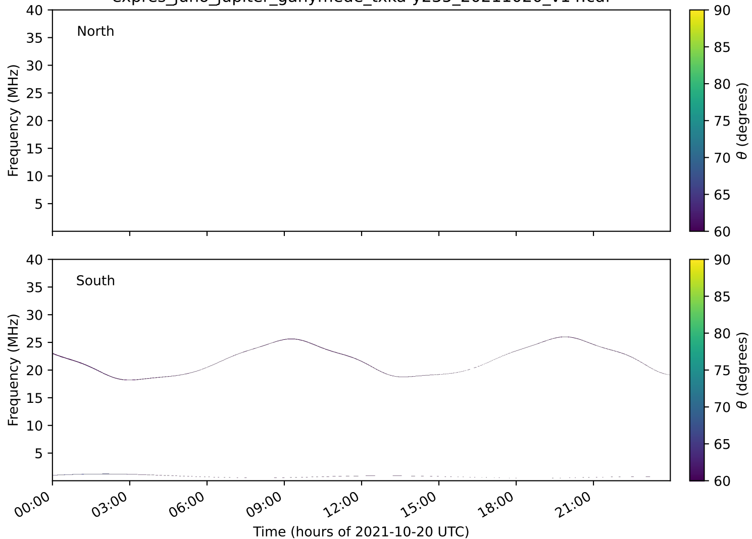
expres_juno_jupiter_ganymede_txka-y235_20211020_v14.cdf
