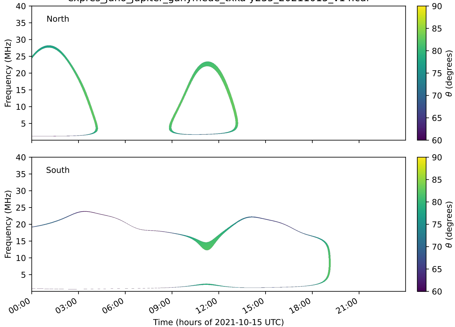
expres_juno_jupiter_ganymede_txka-y235_20211015_v14.cdf
