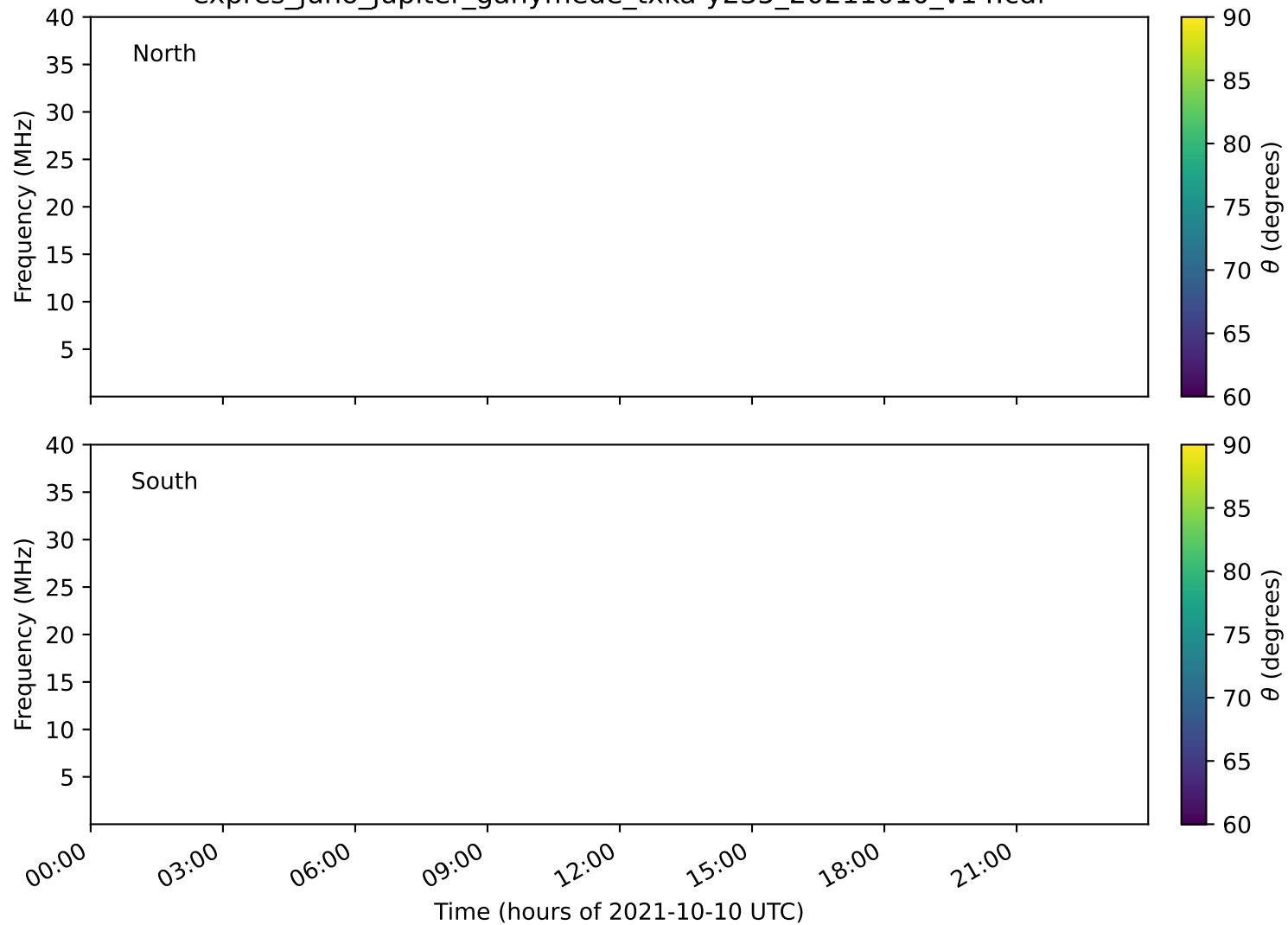
expres_juno_jupiter_ganymede_txka-y235_20211010_v14.cdf
