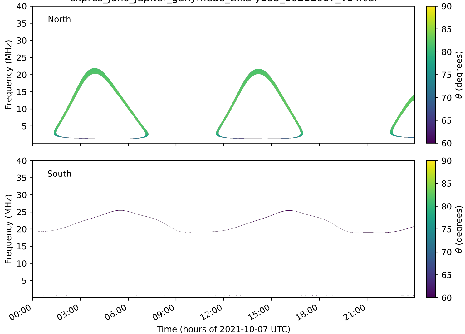
expres_juno_jupiter_ganymede_txka-y235_20211007_v14.cdf
