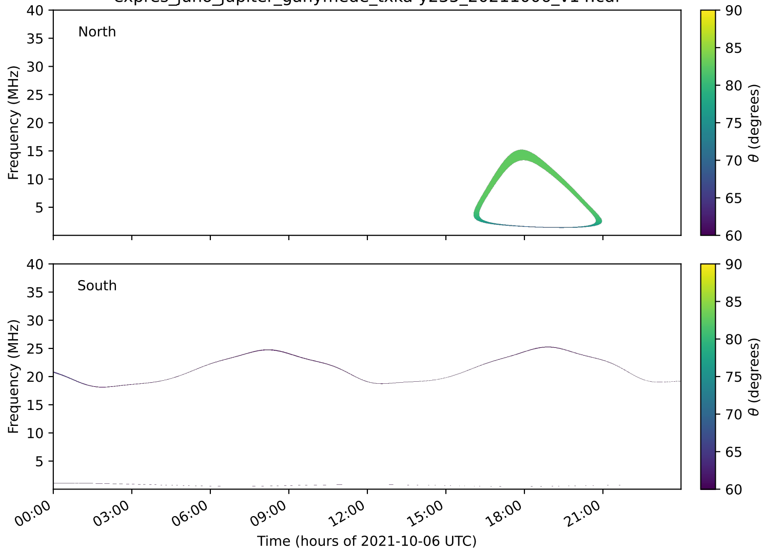
expres_juno_jupiter_ganymede_txka-y235_20211006_v14.cdf
