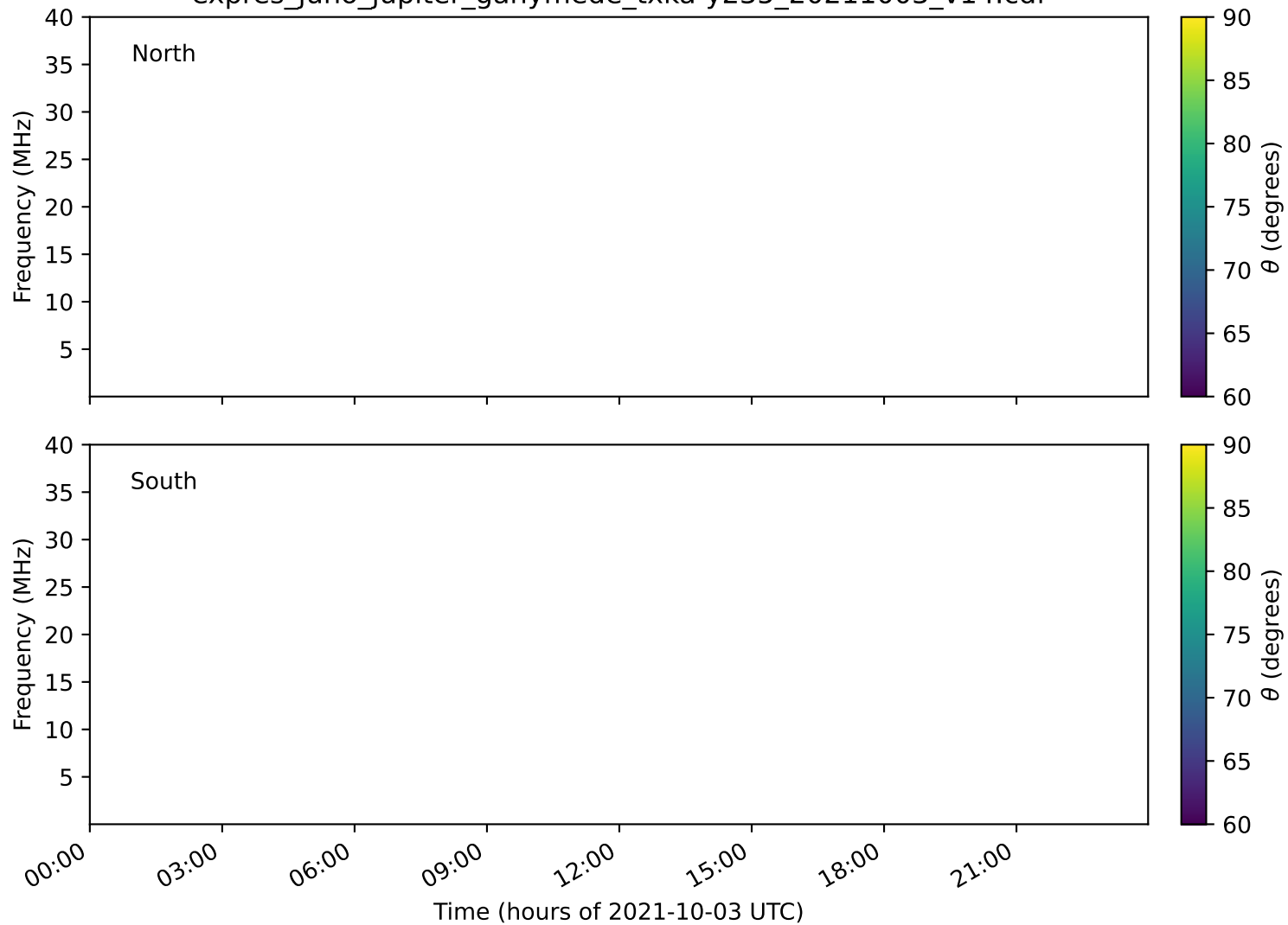
expres_juno_jupiter_ganymede_txka-y235_20211003_v14.cdf
