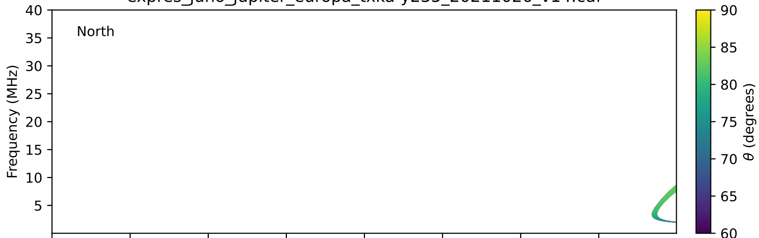
expres_juno_jupiter_europa_txka-y235_20211026_v14.cdf
