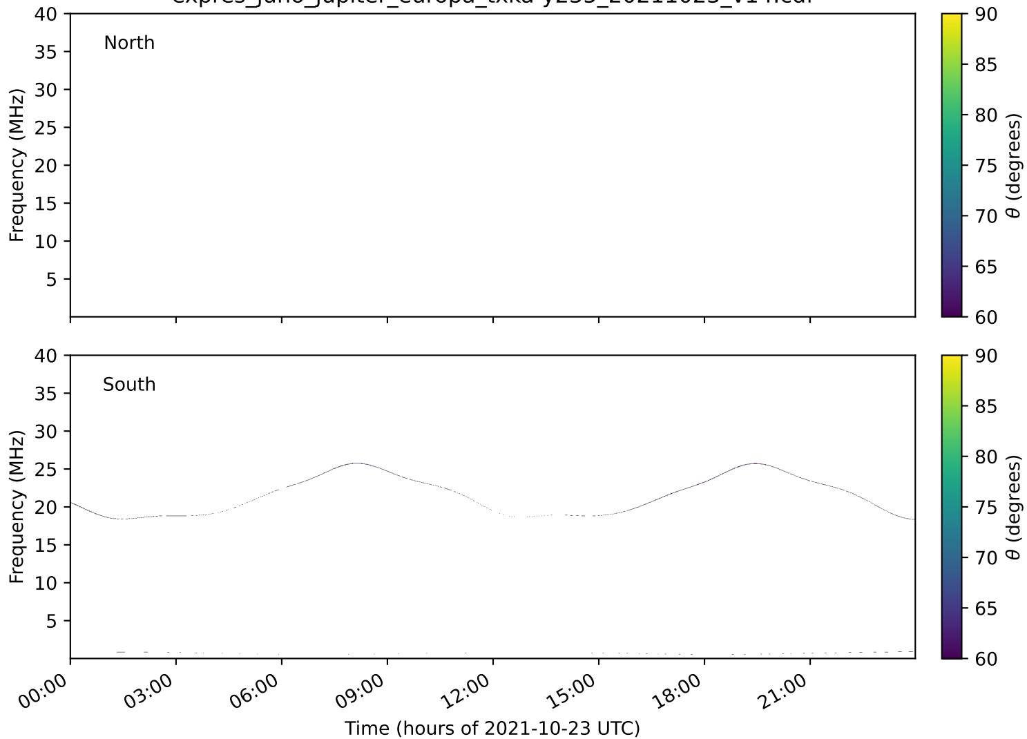
expres_juno_jupiter_europa_txka-y235_20211023_v14.cdf
