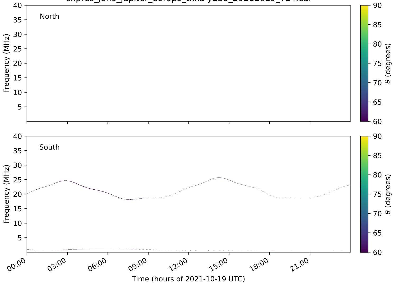
expres_juno_jupiter_europa_txka-y235_20211019_v14.cdf
