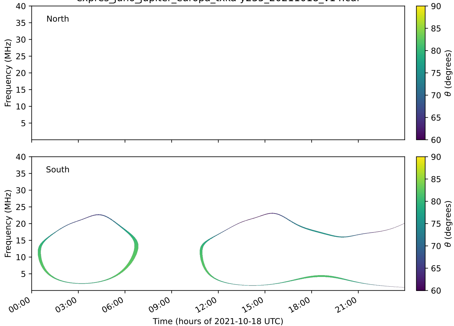
expres_juno_jupiter_europa_txka-y235_20211018_v14.cdf
