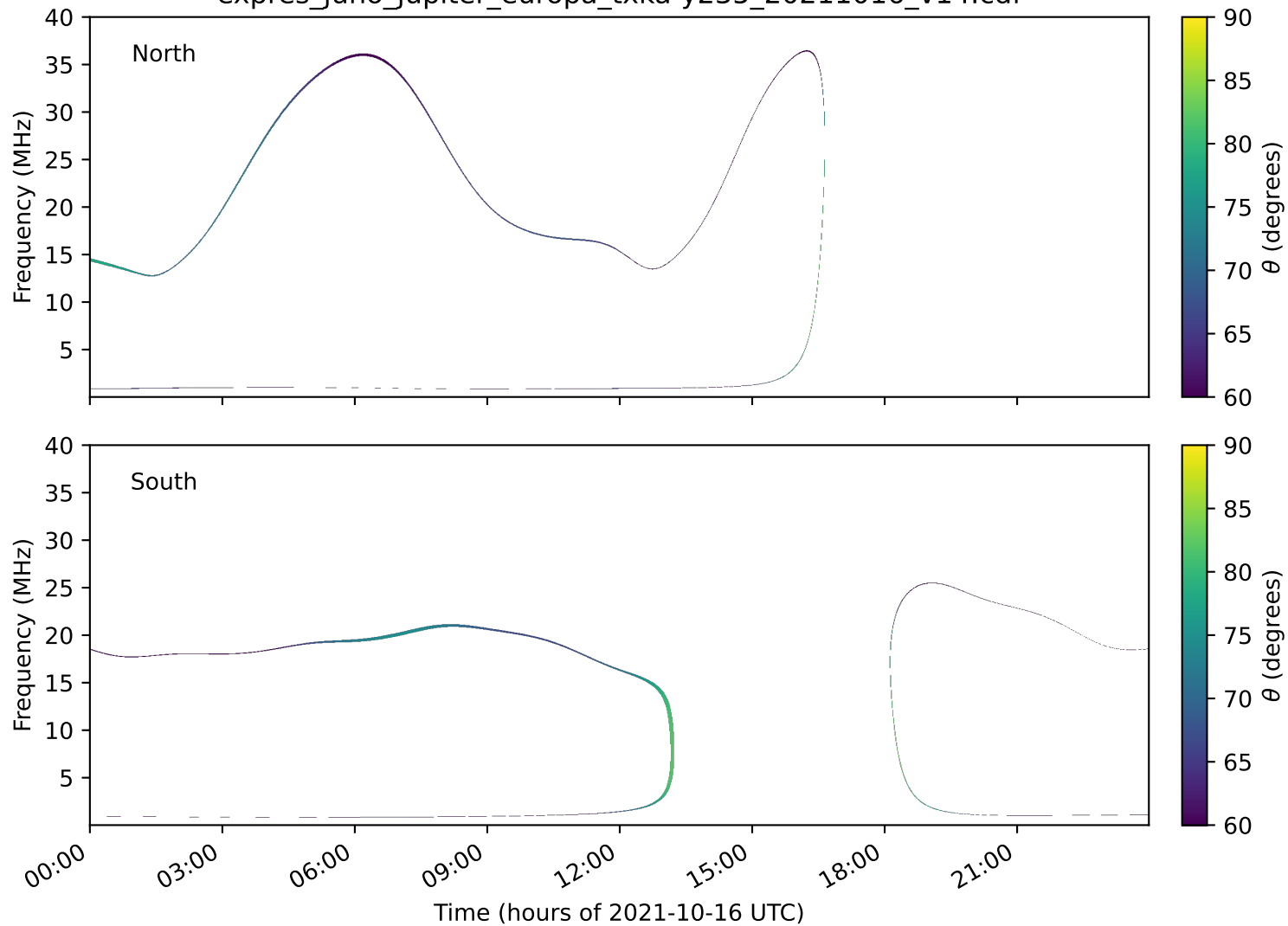
expres_juno_jupiter_europa_txka-y235_20211016_v14.cdf
